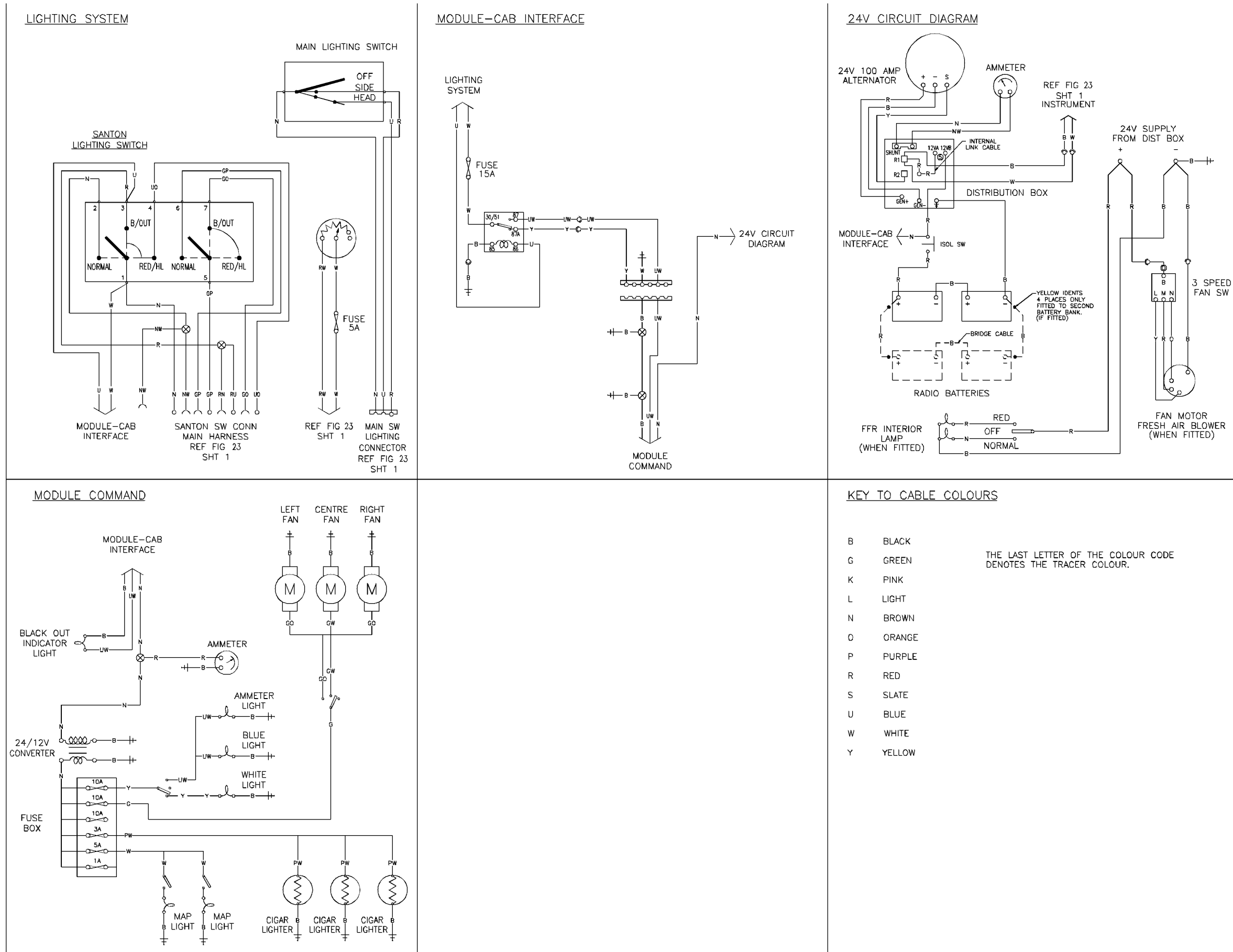
Figure 30 – Mortar Carrier FFR Wiring Schematic
