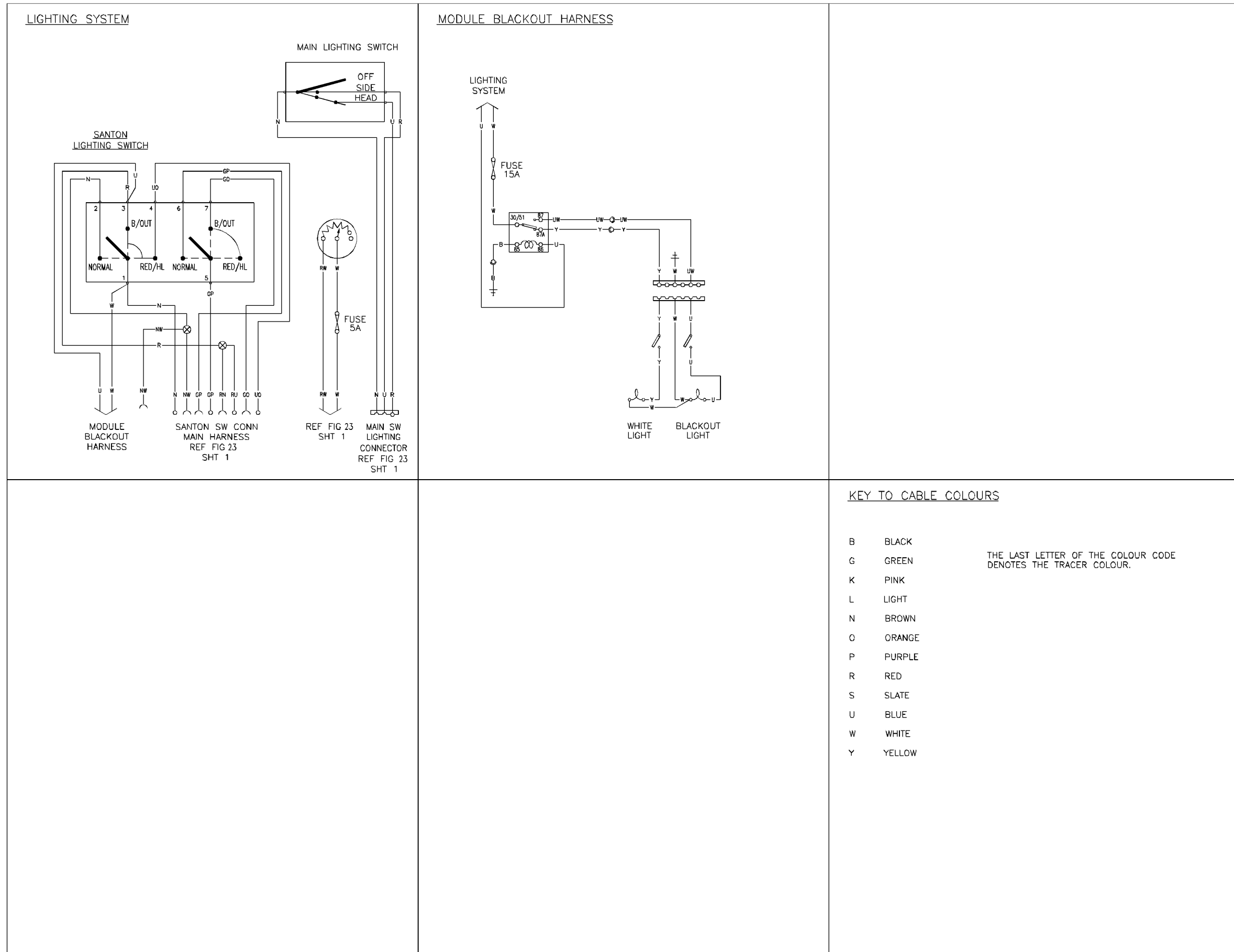
Figure 29 – Assault Wiring Schematic
