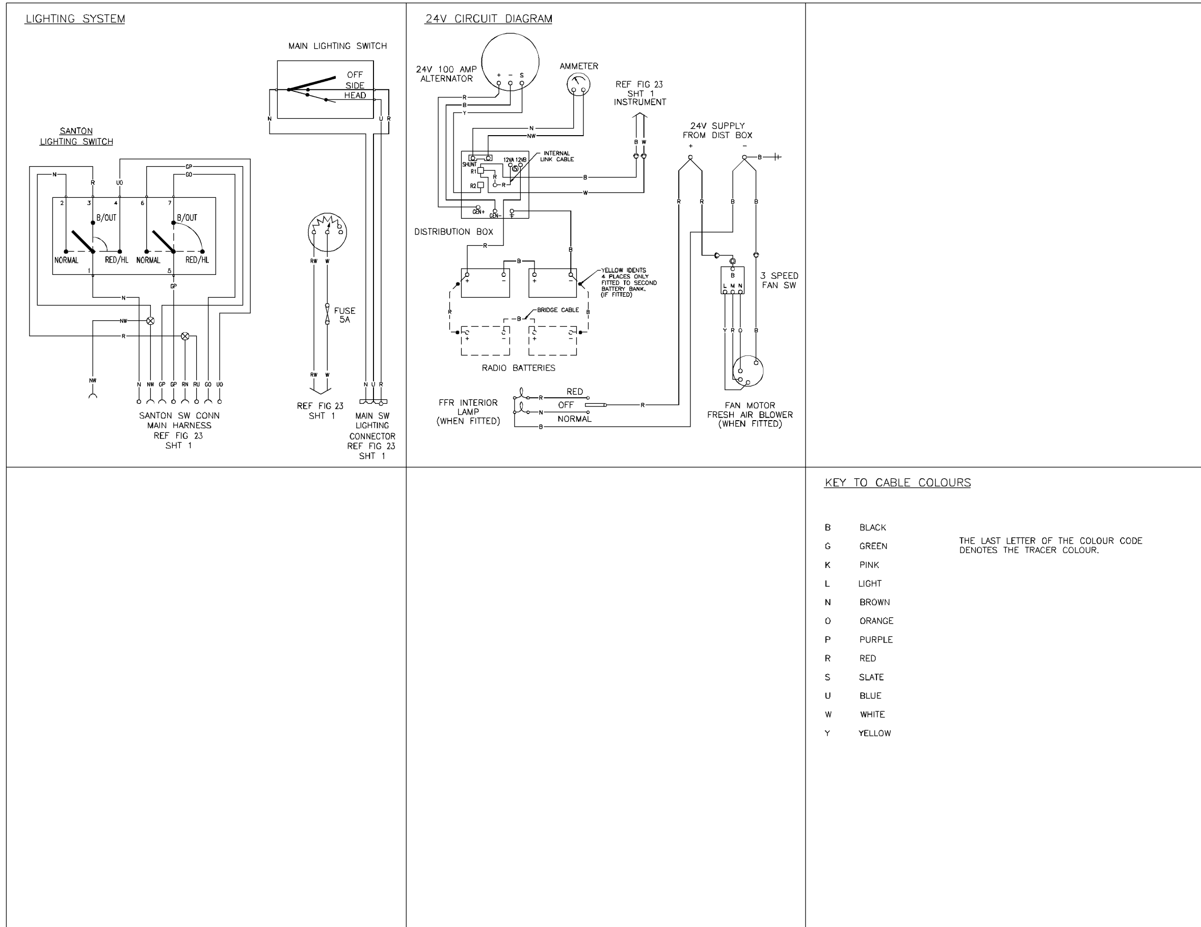
Figure 28 – Infantry Carrier FFR Wiring Schematic
