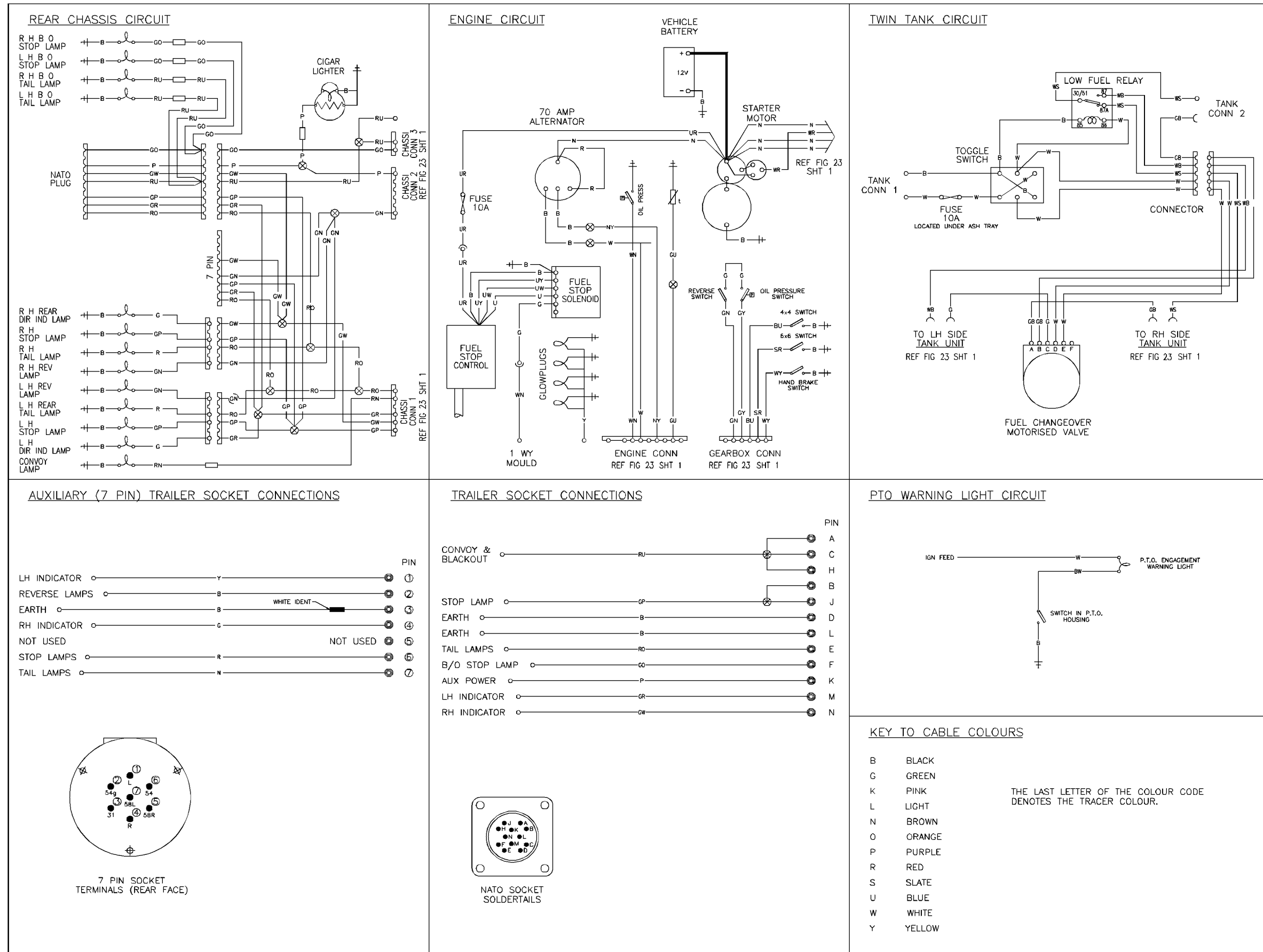
Figure 27 – 6x6 Common Wiring Schematic (Sheet 2 of 2)
