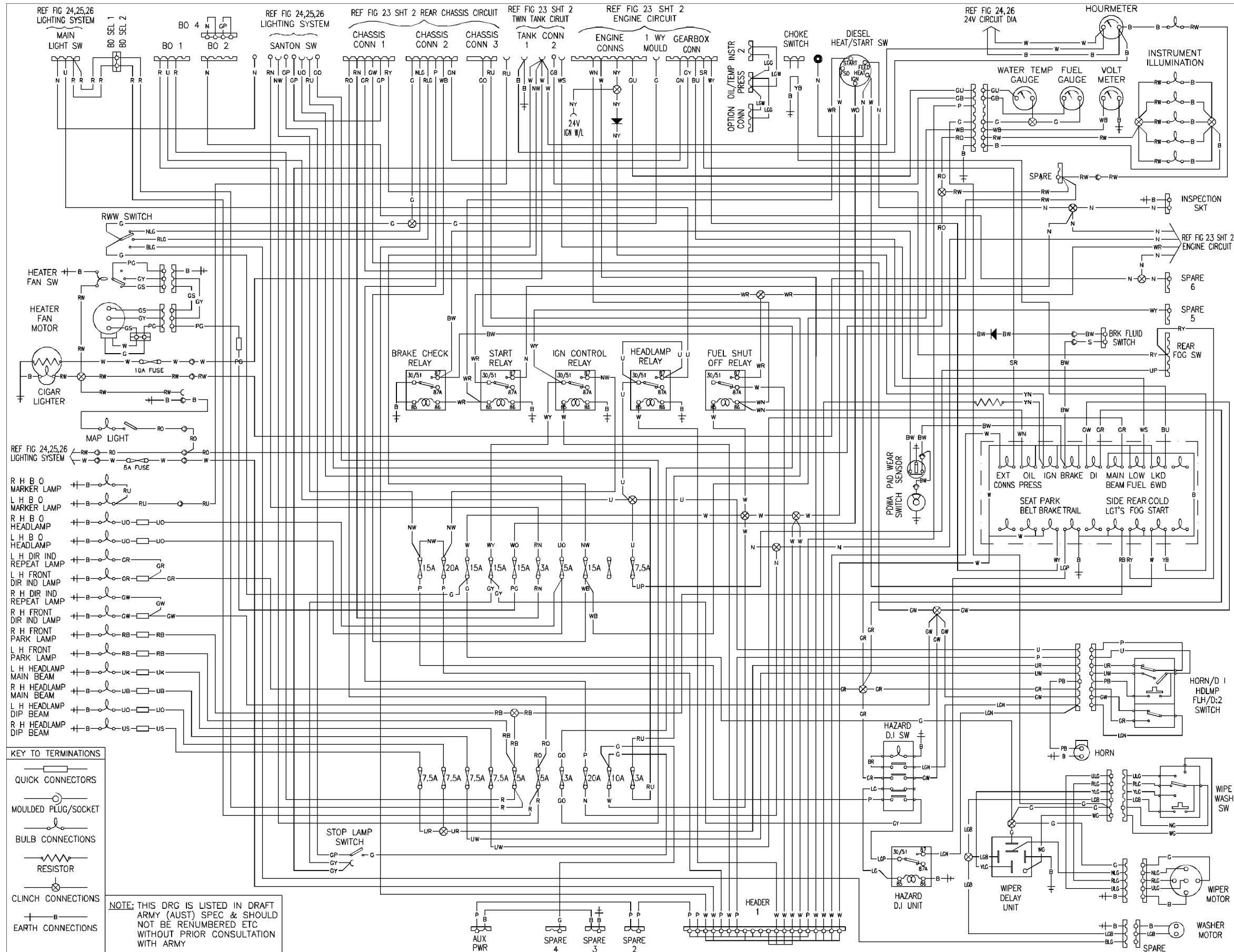
Figure 27 – 6x6 Common Wiring Schematic (Sheet 1 of 2)
