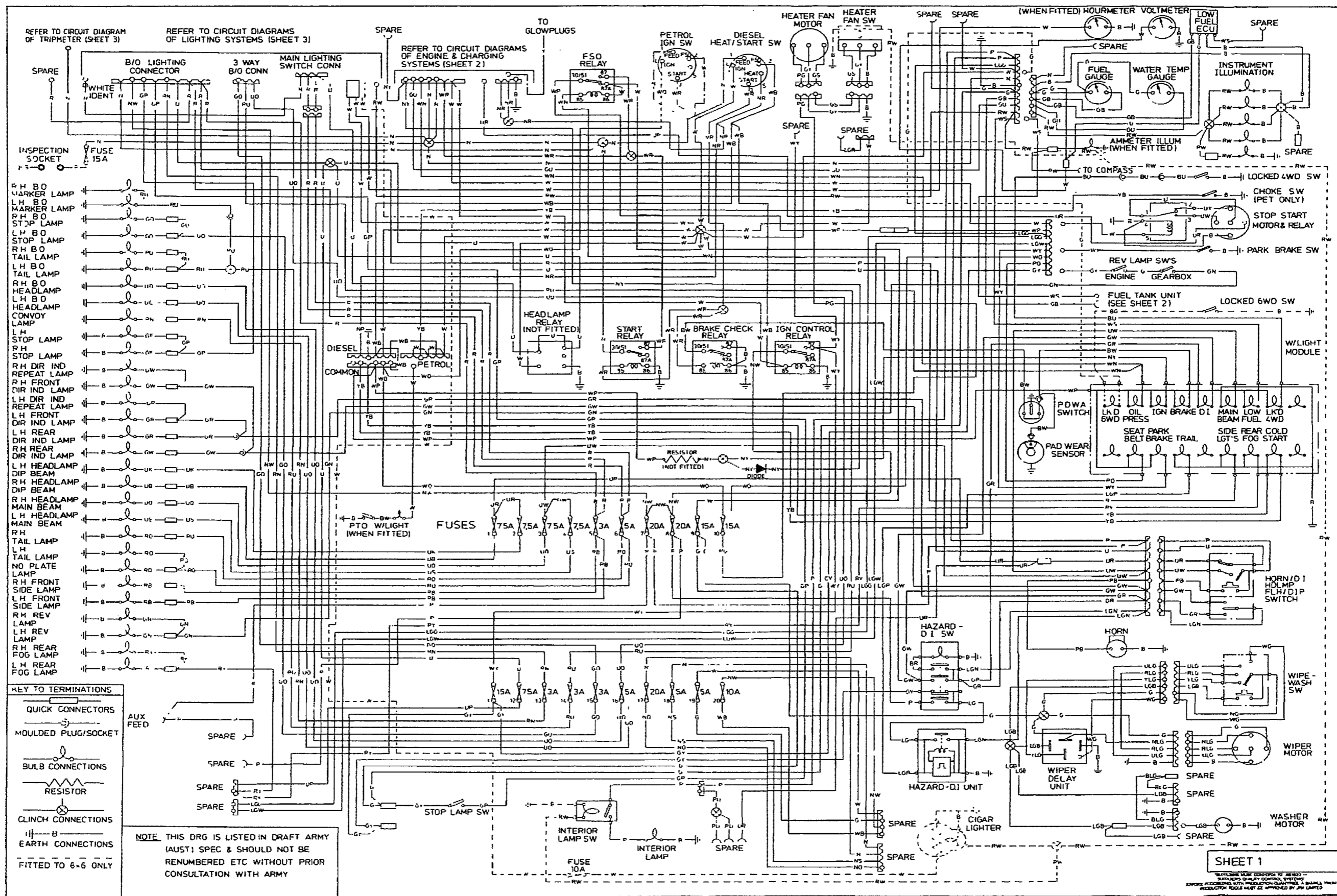
Figure 26 Wiring Diagram (Sheet 1 of 3)
