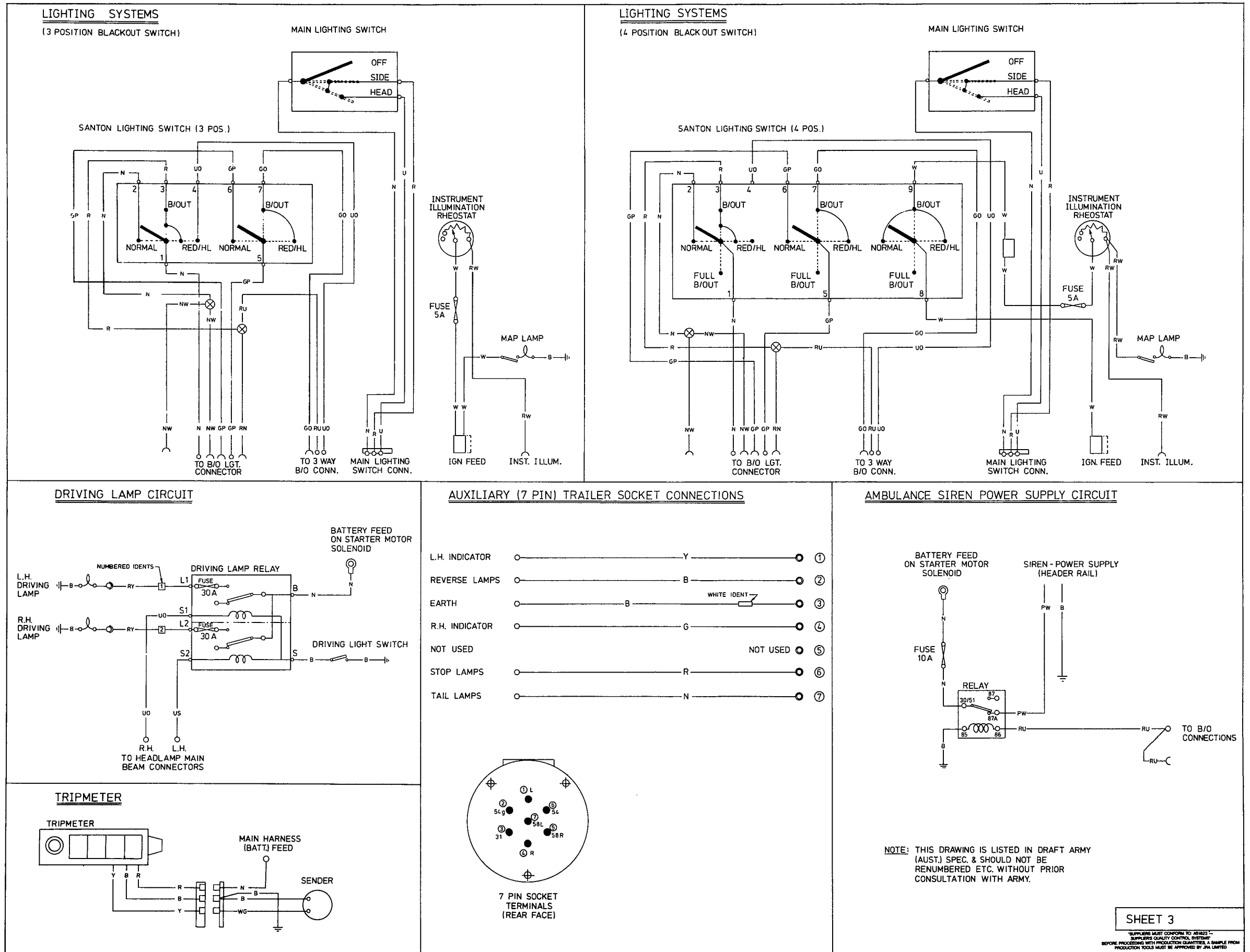
Figure 15 — Wiring Diagram — (Sheet 3)
