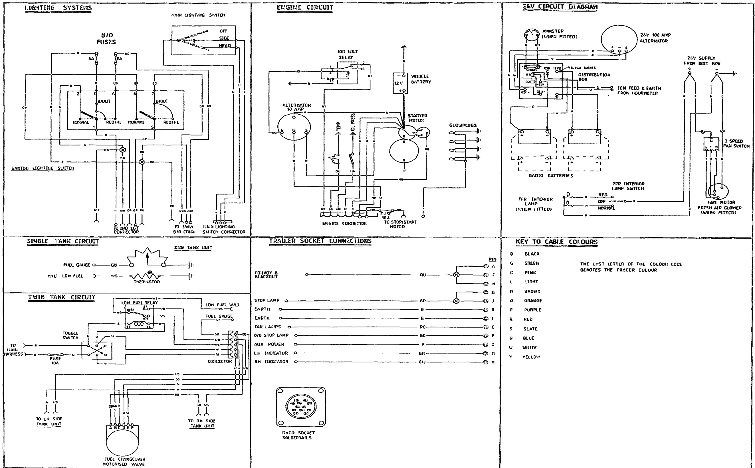
Figure 211 Wiring Diagram (Sheet 3 of 3)
