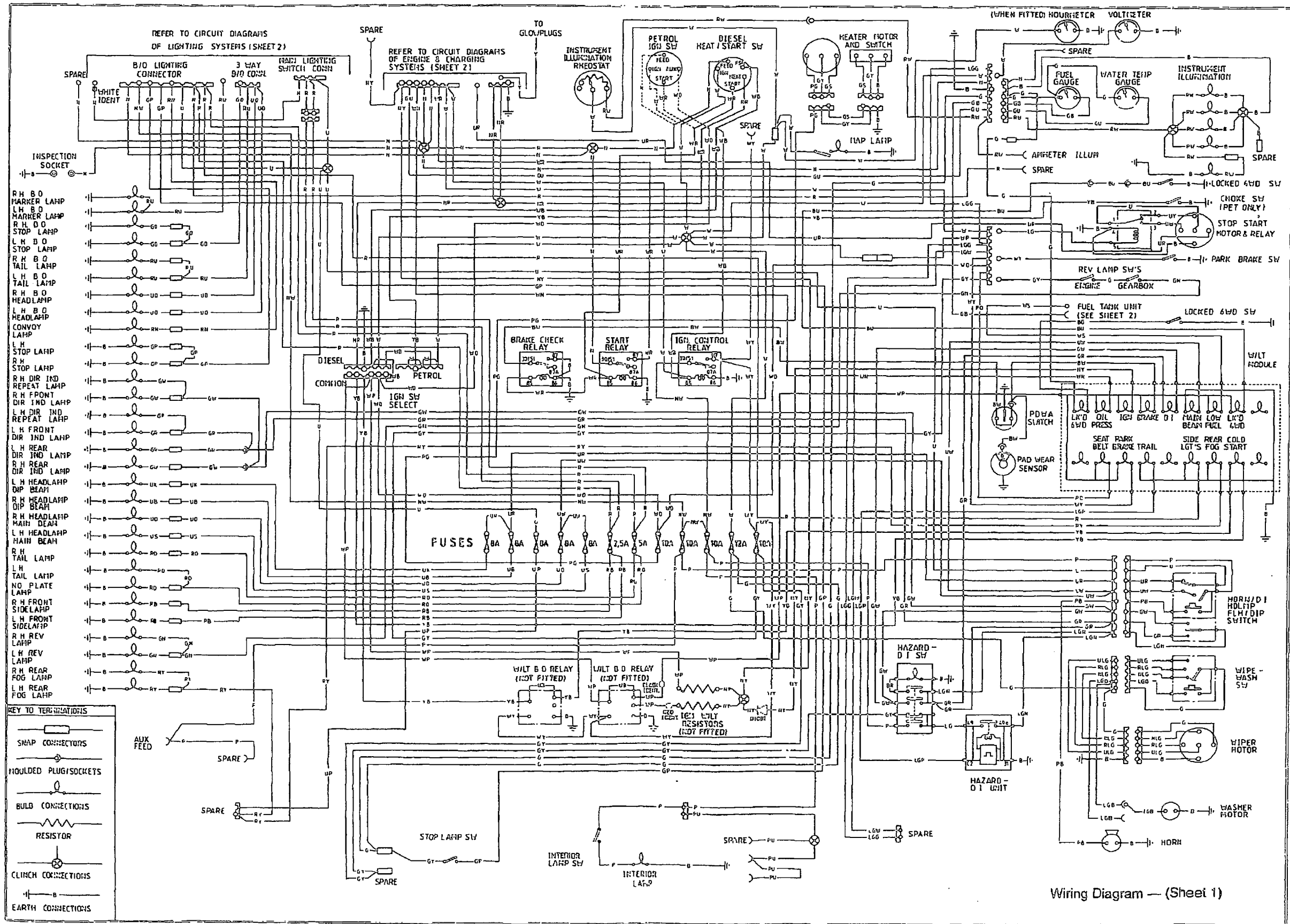
Figure 211 Wiring Diagram (Sheet 1 of 1)
