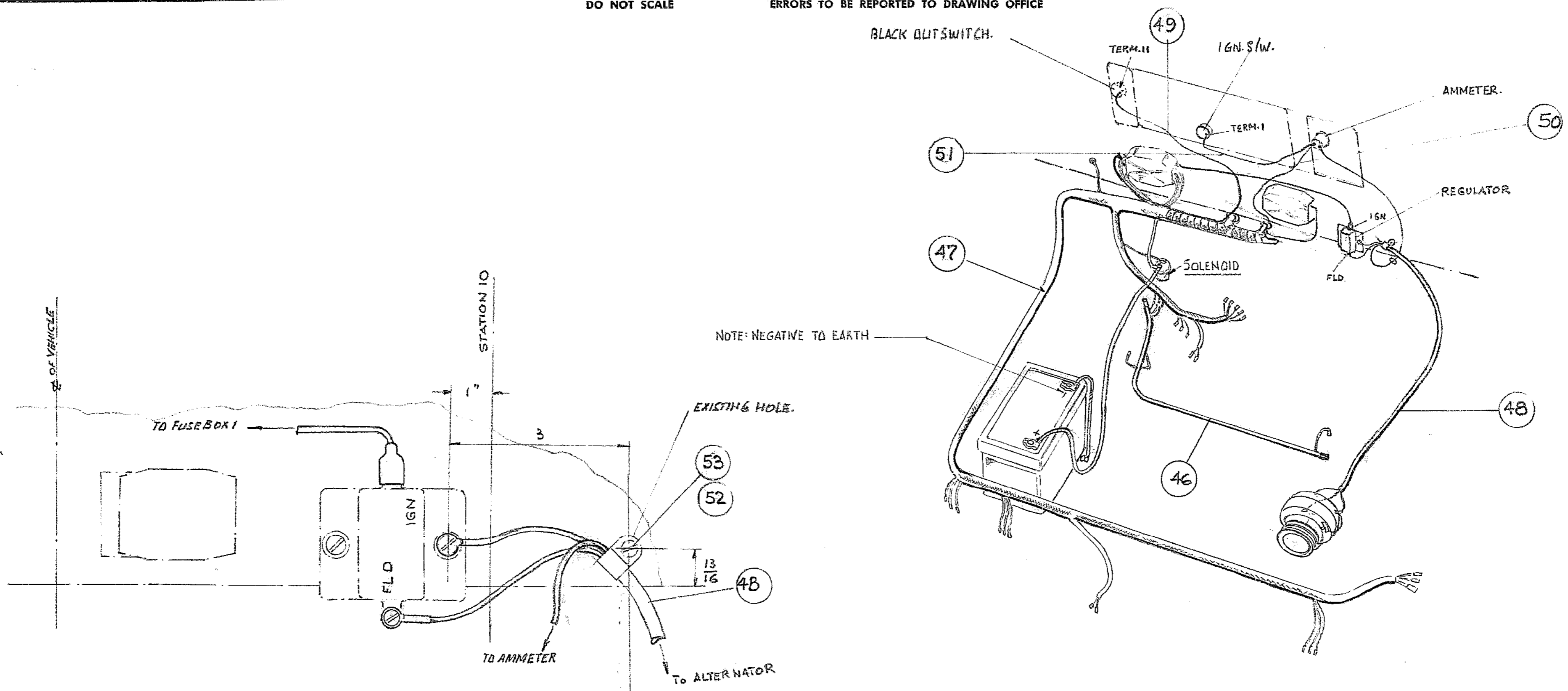
SCRAP VIEW OF DASH ASSEMBLY NOTE :- VIEW LOOKING FROM ENGINE COMPARTMENT
